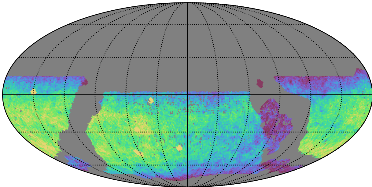
mw_roll_bulge_v3.3_10yrs WFD u band: CoaddM5
