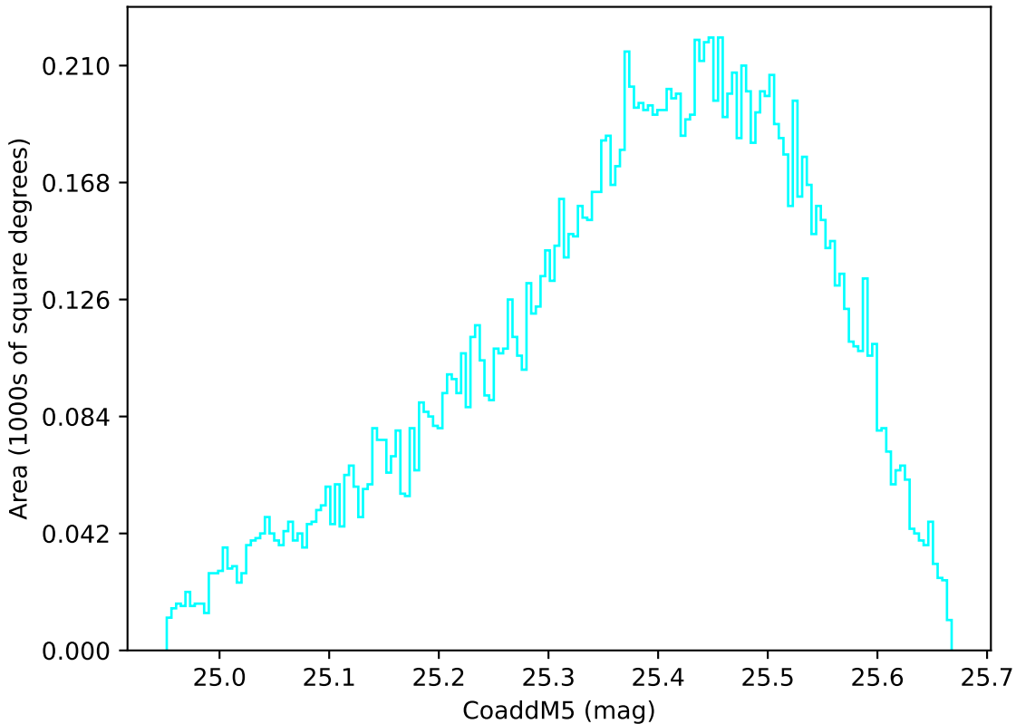
mw_roll_bulge_v3.3_10yrs WFD u band: CoaddM5
