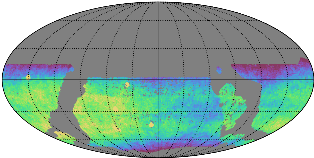
mw_roll_bulge_v3.3_10yrs WFD r band: CoaddM5
