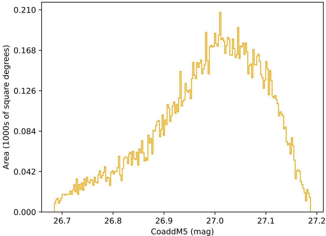
mw_roll_bulge_v3.3_10yrs WFD r band: CoaddM5
