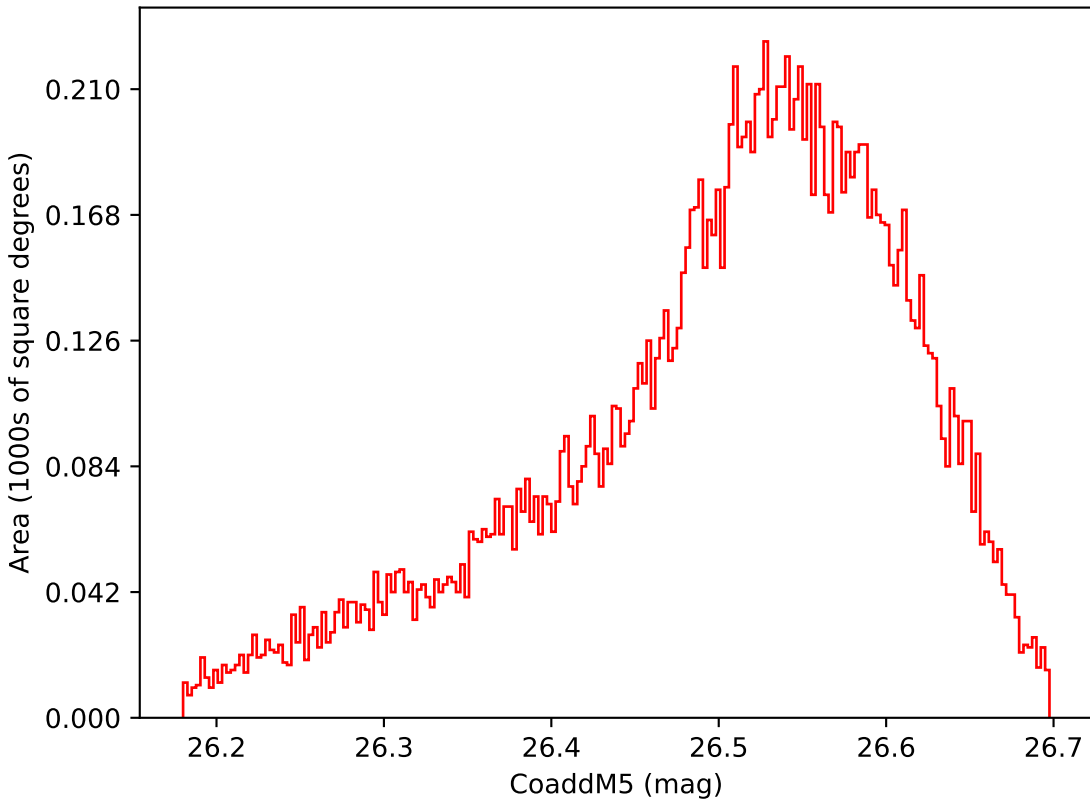
mw_roll_bulge_v3.3_10yrs WFD i band: CoaddM5
