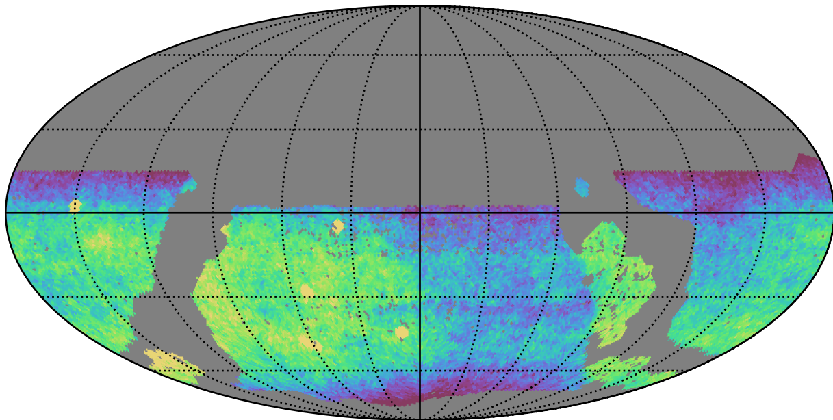
mw_roll_bulge_v3.3_10yrs WFD g band: CoaddM5
