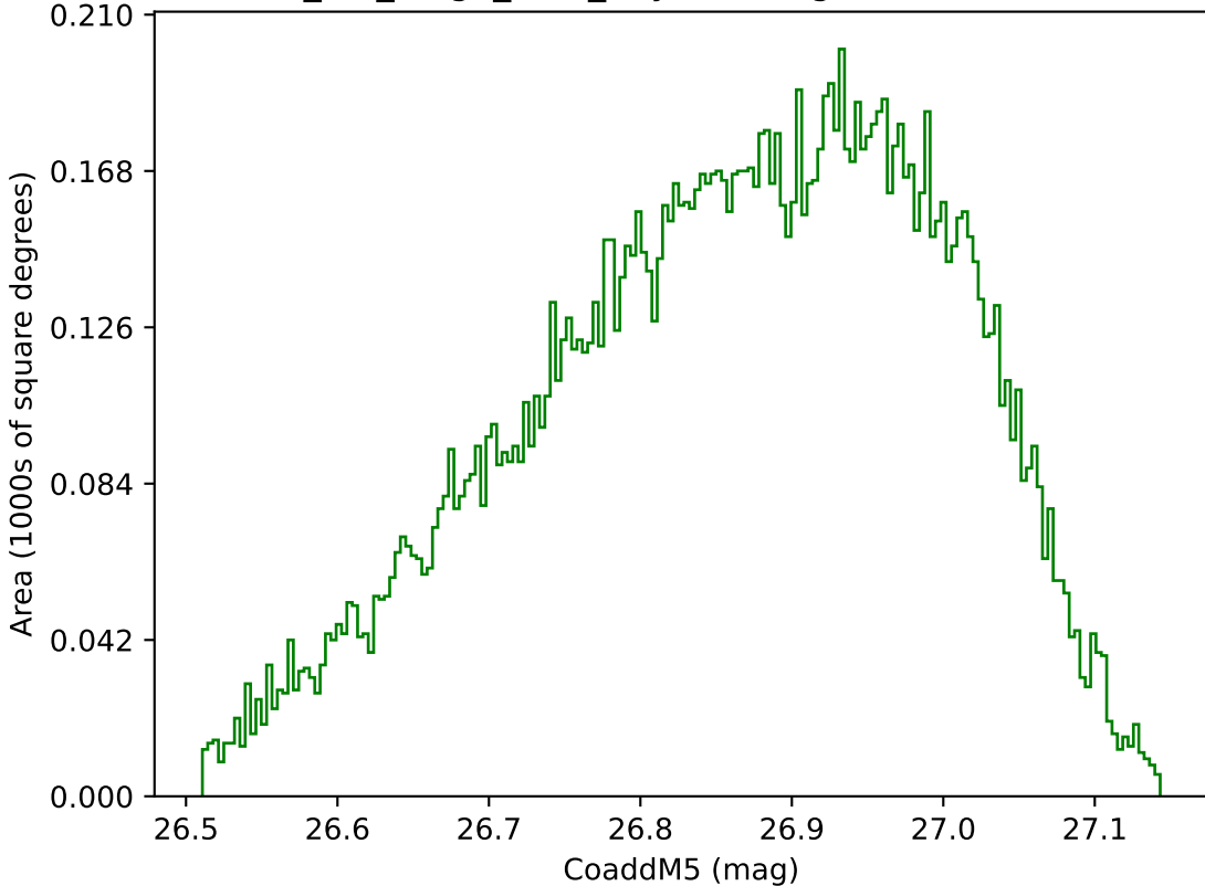
mw_roll_bulge_v3.3_10yrs WFD g band: CoaddM5
