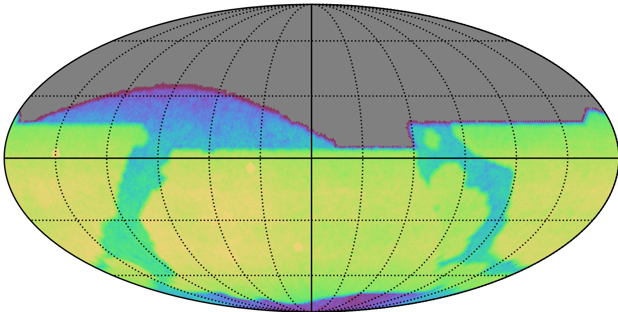
mw_roll_bulge_v3.3_10yrs All sky z band: CoaddM5
