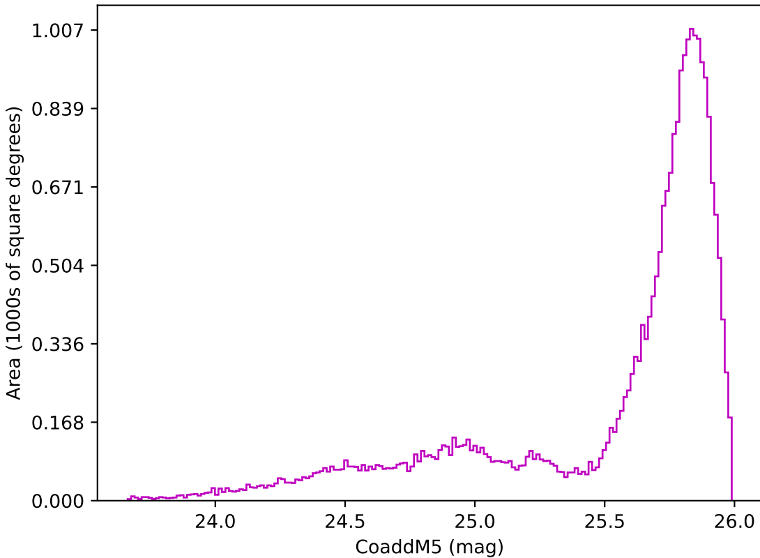
mw_roll_bulge_v3.3_10yrs All sky z band: CoaddM5
