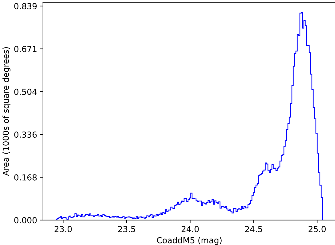
mw_roll_bulge_v3.3_10yrs All sky y band: CoaddM5
