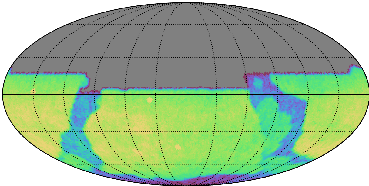
mw_roll_bulge_v3.3_10yrs All sky u band: CoaddM5
