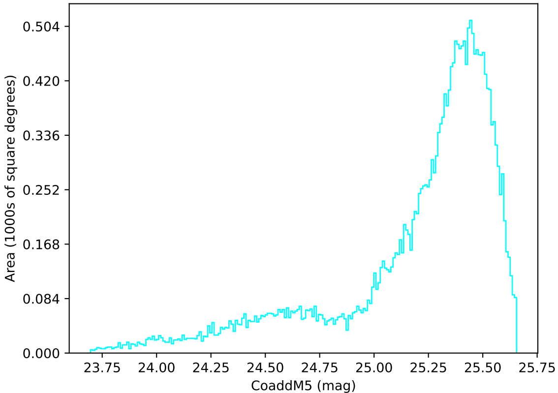
mw_roll_bulge_v3.3_10yrs All sky u band: CoaddM5
