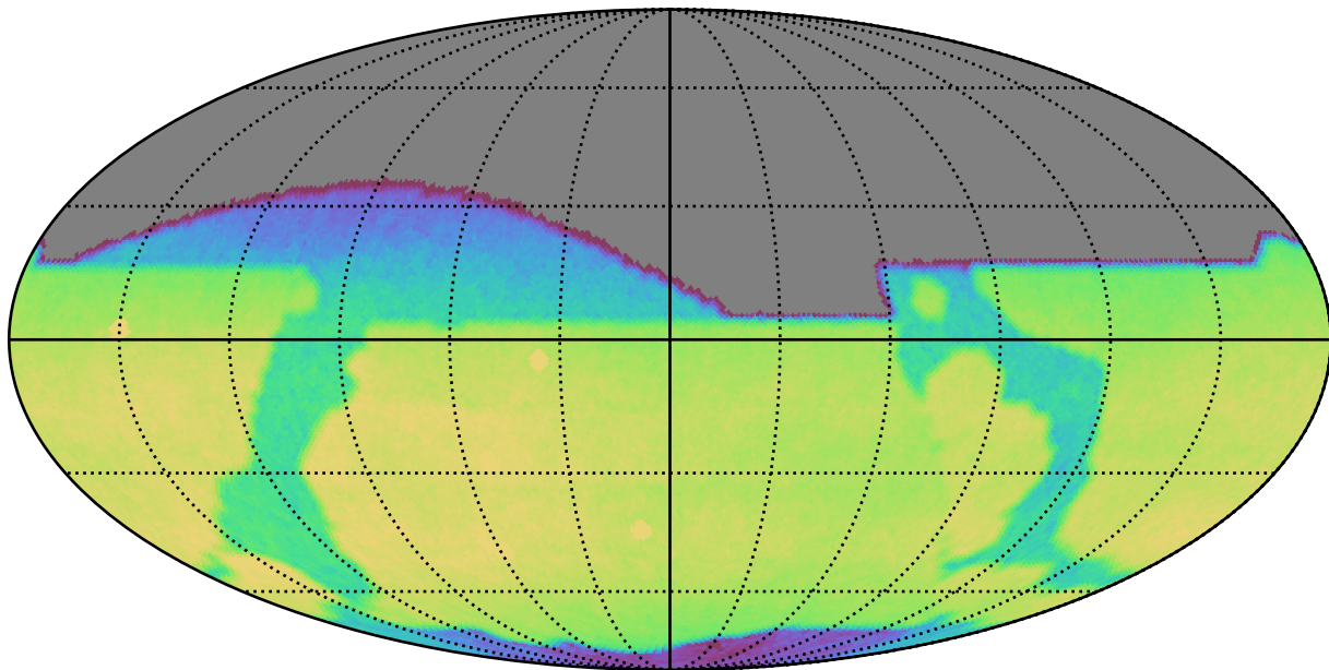
mw_roll_bulge_v3.3_10yrs All sky r band: CoaddM5
