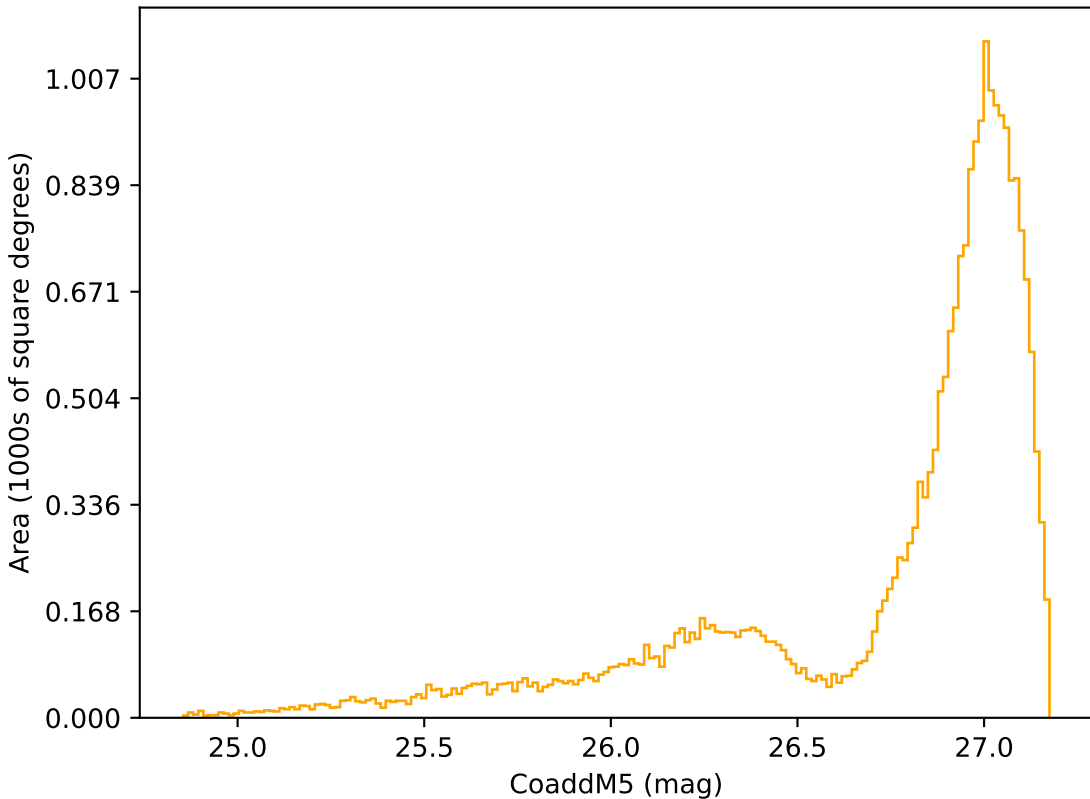
mw_roll_bulge_v3.3_10yrs All sky r band: CoaddM5
