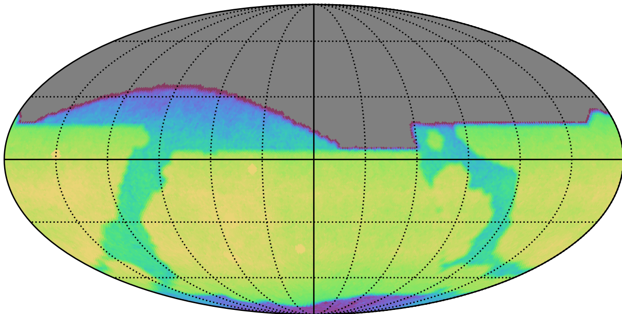
mw_roll_bulge_v3.3_10yrs All sky i band: CoaddM5
