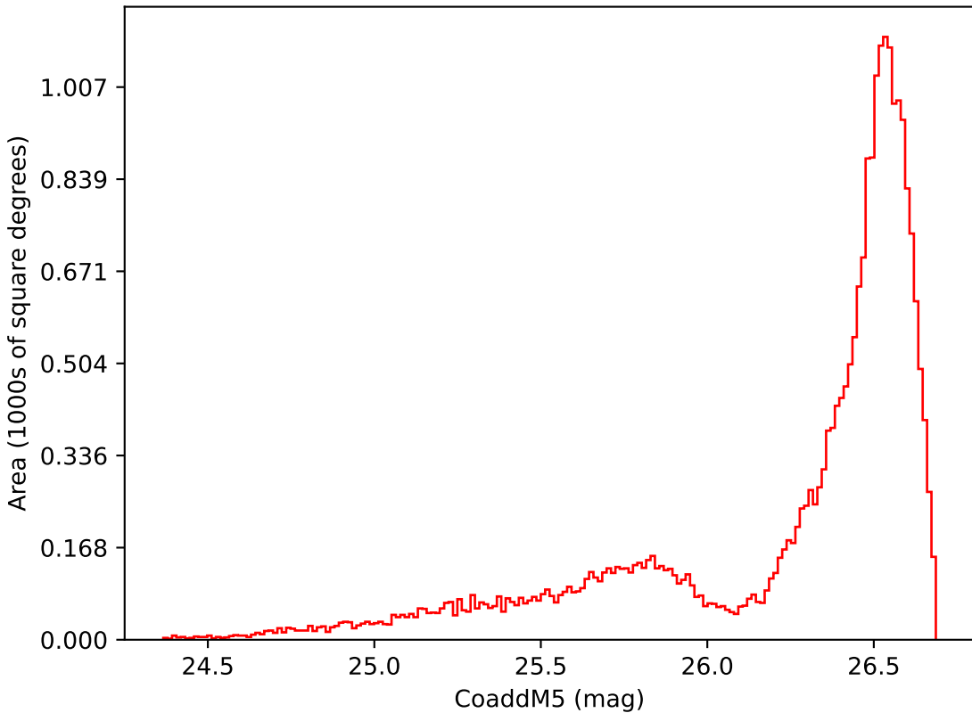
mw_roll_bulge_v3.3_10yrs All sky i band: CoaddM5
