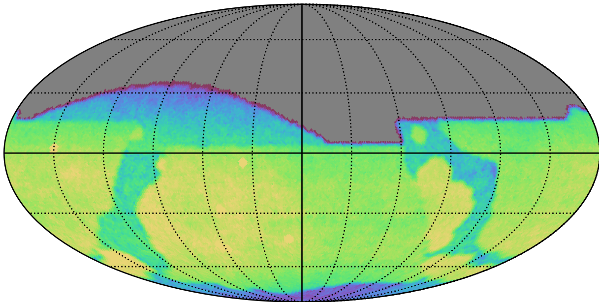
mw_roll_bulge_v3.3_10yrs All sky g band: CoaddM5
