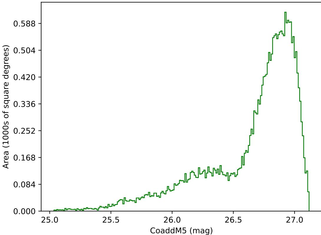
mw_roll_bulge_v3.3_10yrs All sky g band: CoaddM5
