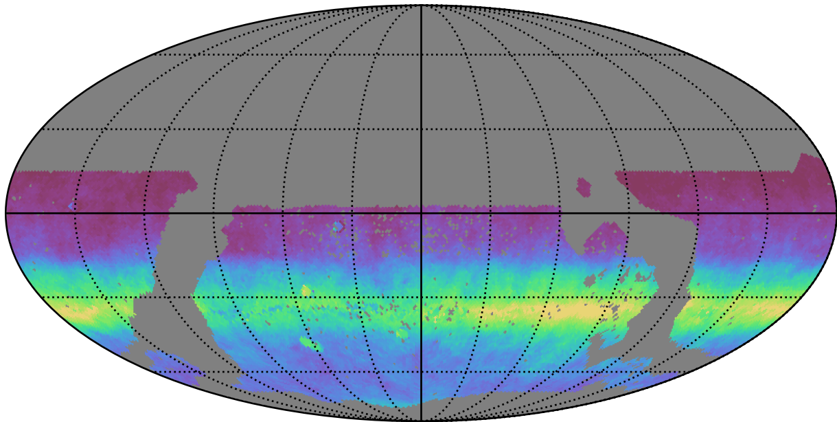
mw_roll_bulge_v3.3_10yrs WFD all bands: AngleRms rotSkyPos
