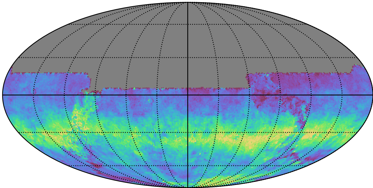
mw_roll_bulge_v3.3_10yrs All sky u band: AngleRms rotSkyPos
