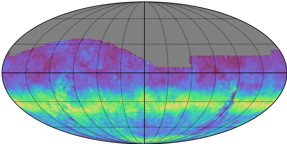
mw_roll_bulge_v3.3_10yrs All sky g band: AngleRms rotSkyPos
