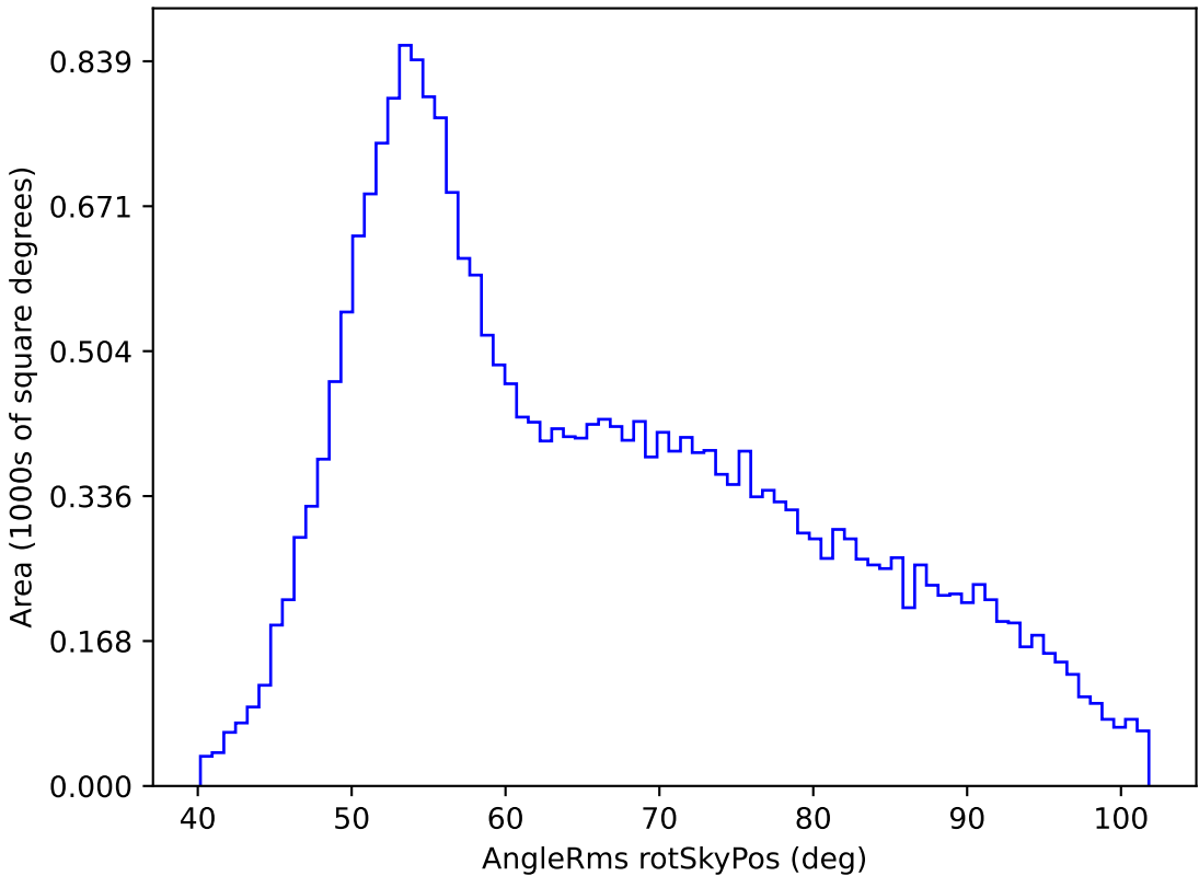
mw_roll_bulge_v3.3_10yrs All sky g band: AngleRms rotSkyPos
