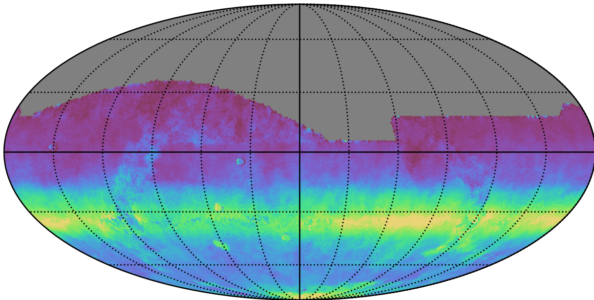
mw_roll_bulge_v3.3_10yrs All sky all bands: AngleRms rotSkyPos
