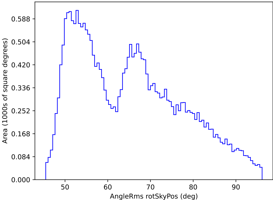
mw_roll_bulge_v3.3_10yrs All sky all bands: AngleRms rotSkyPos
