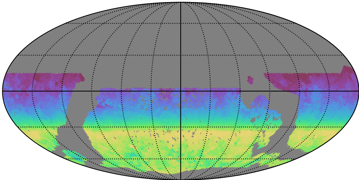
mw_roll_bulge_v3.3_10yrs WFD all bands: AngleRange rotSkyPos
