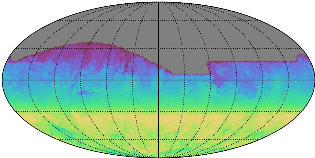
mw_roll_bulge_v3.3_10yrs All sky all bands: AngleRange rotSkyPos
