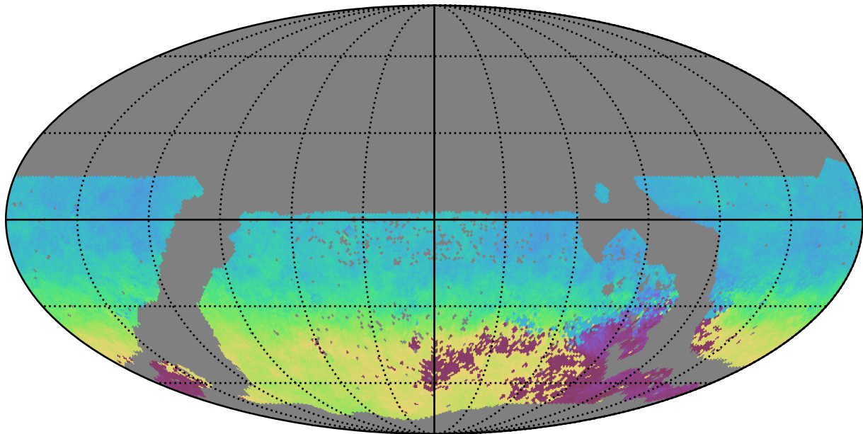
mw_roll_bulge_v3.3_10yrs WFD u band: AngleMean rotSkyPos
