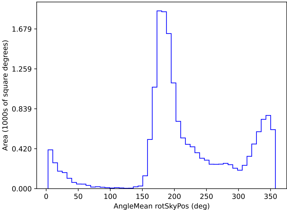
mw_roll_bulge_v3.3_10yrs WFD u band: AngleMean rotSkyPos
