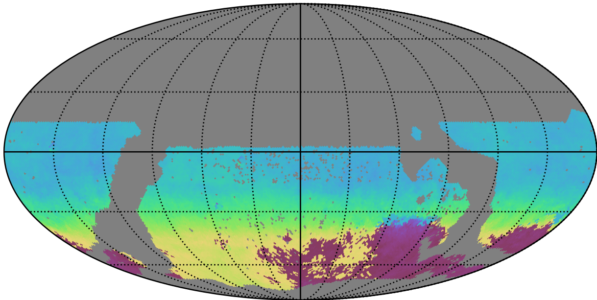
mw_roll_bulge_v3.3_10yrs WFD r band: AngleMean rotSkyPos
