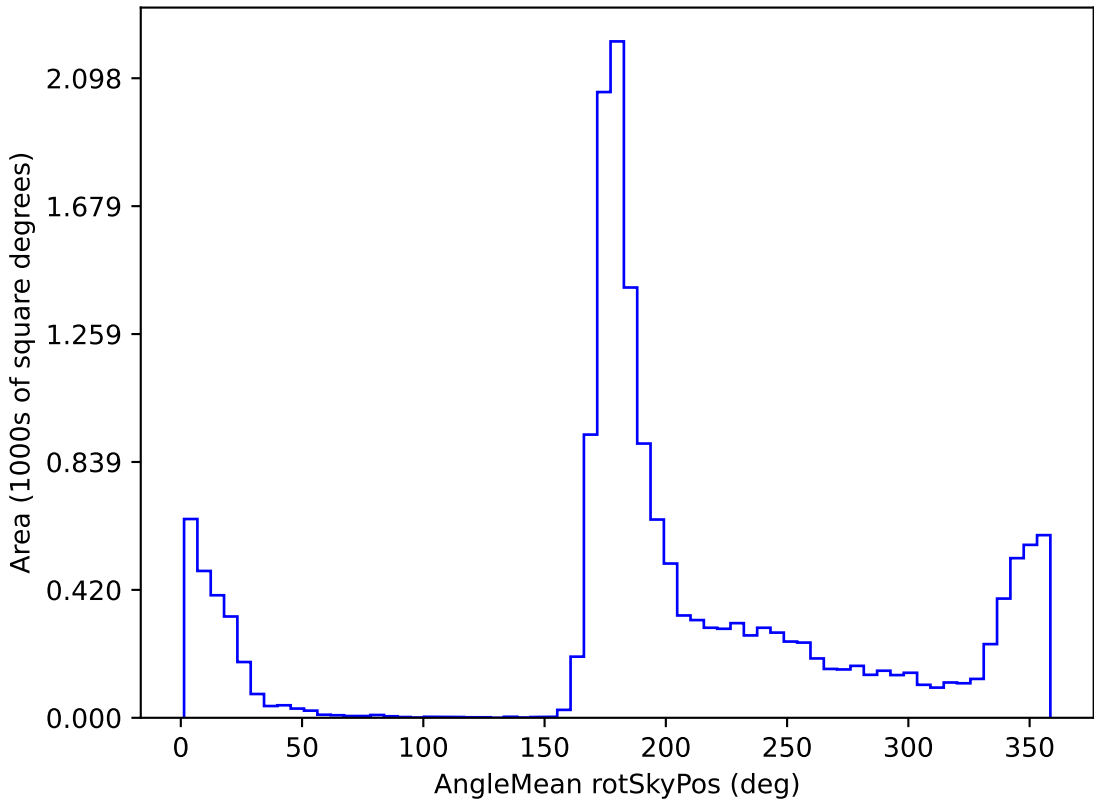
mw_roll_bulge_v3.3_10yrs WFD r band: AngleMean rotSkyPos
