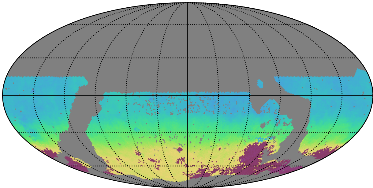
mw_roll_bulge_v3.3_10yrs WFD i band: AngleMean rotSkyPos
