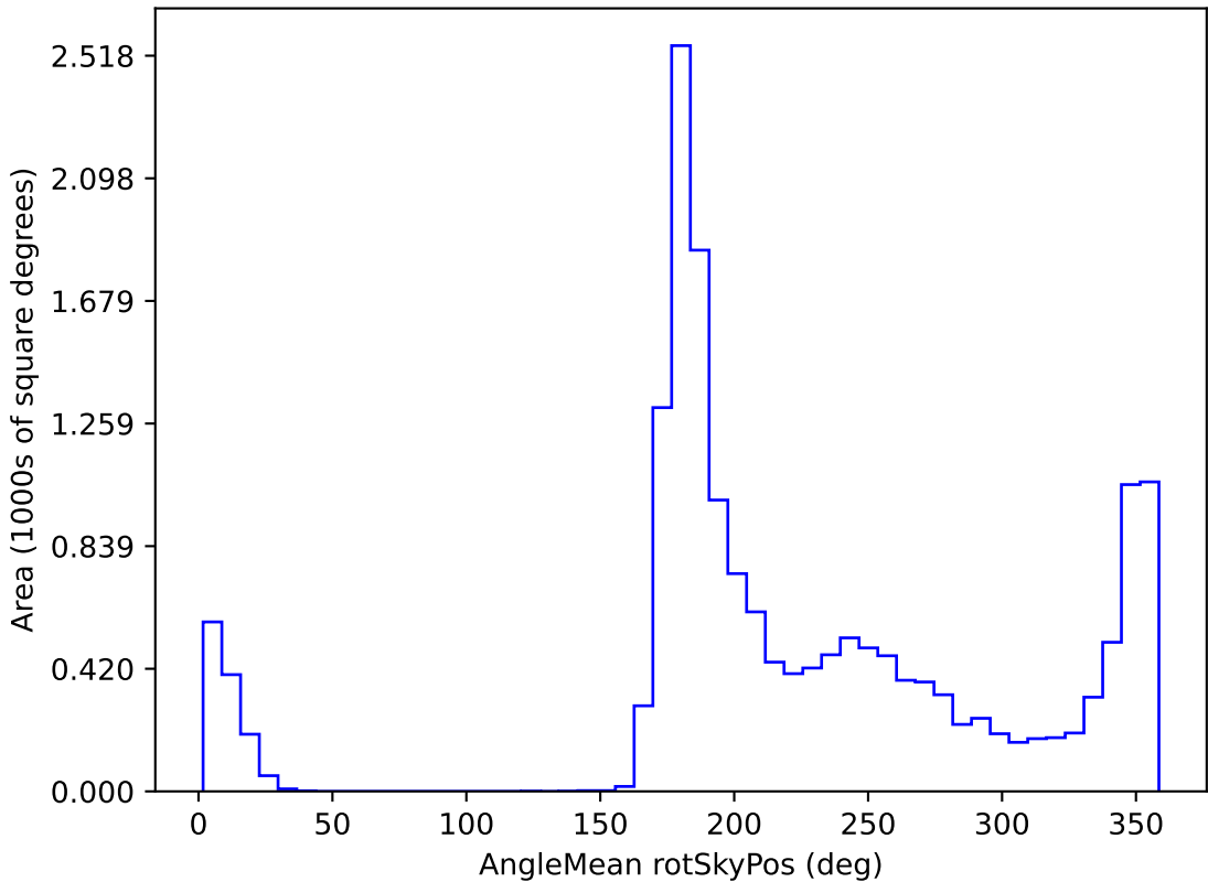
mw_roll_bulge_v3.3_10yrs WFD i band: AngleMean rotSkyPos
