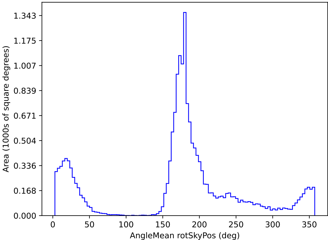
mw_roll_bulge_v3.3_10yrs WFD g band: AngleMean rotSkyPos
