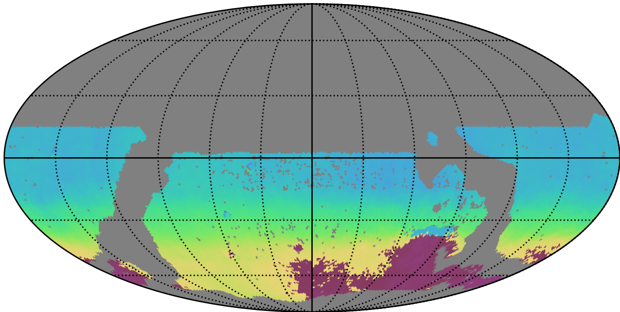
mw_roll_bulge_v3.3_10yrs WFD all bands: AngleMean rotSkyPos
