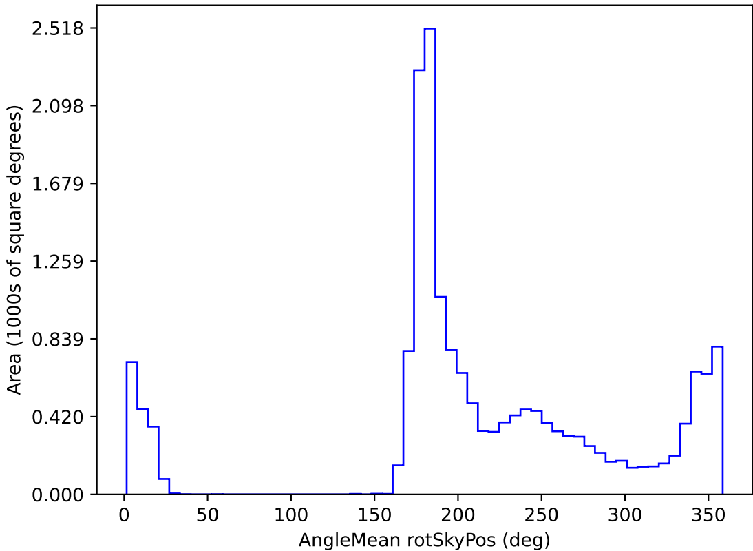
mw_roll_bulge_v3.3_10yrs WFD all bands: AngleMean rotSkyPos
