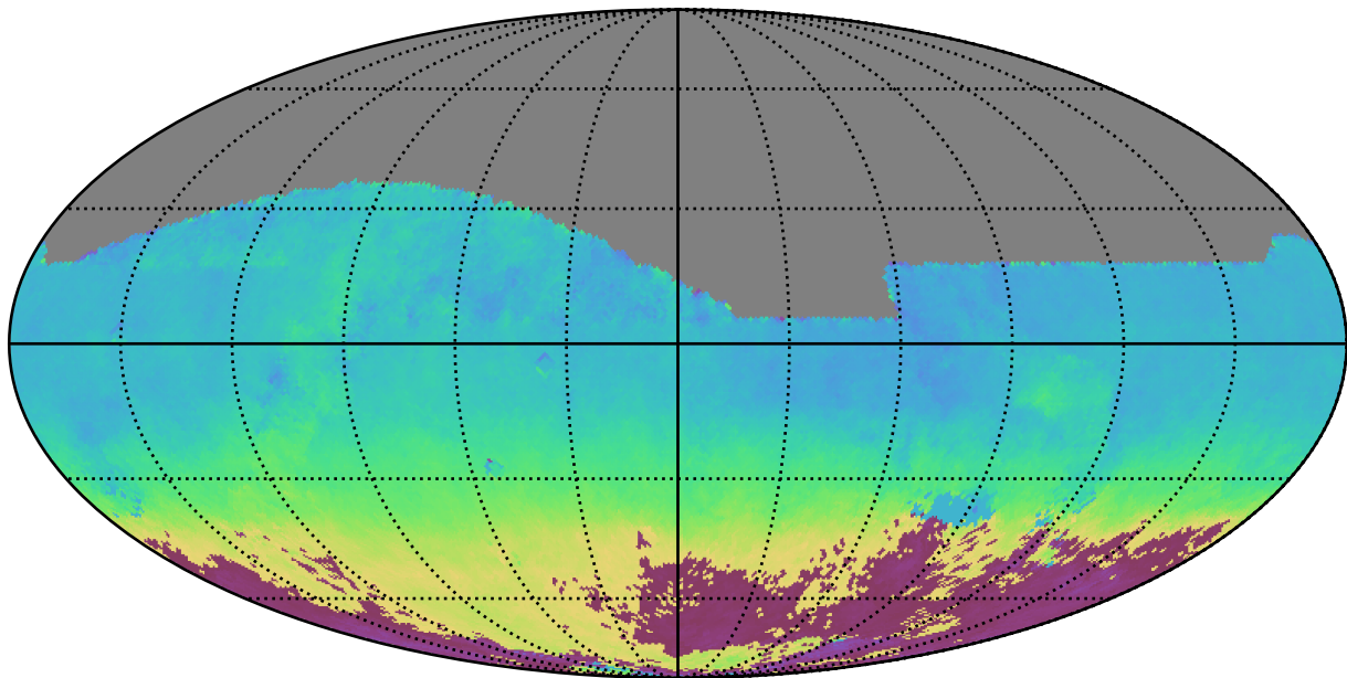
mw_roll_bulge_v3.3_10yrs All sky z band: AngleMean rotSkyPos
