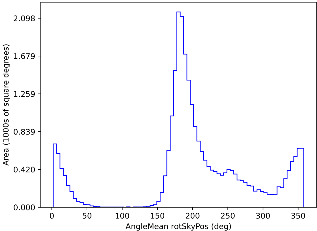
mw_roll_bulge_v3.3_10yrs All sky z band: AngleMean rotSkyPos
