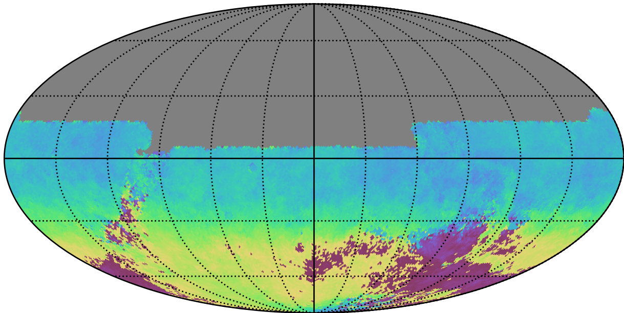
mw_roll_bulge_v3.3_10yrs All sky u band: AngleMean rotSkyPos
