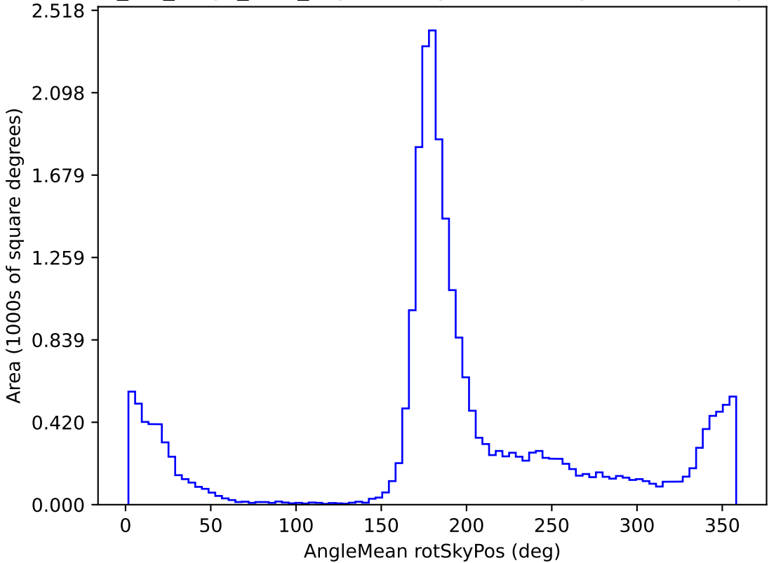
mw_roll_bulge_v3.3_10yrs All sky r band: AngleMean rotSkyPos
