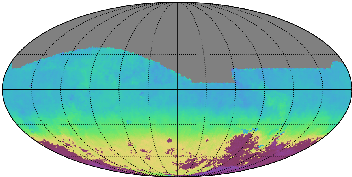
mw_roll_bulge_v3.3_10yrs All sky i band: AngleMean rotSkyPos
