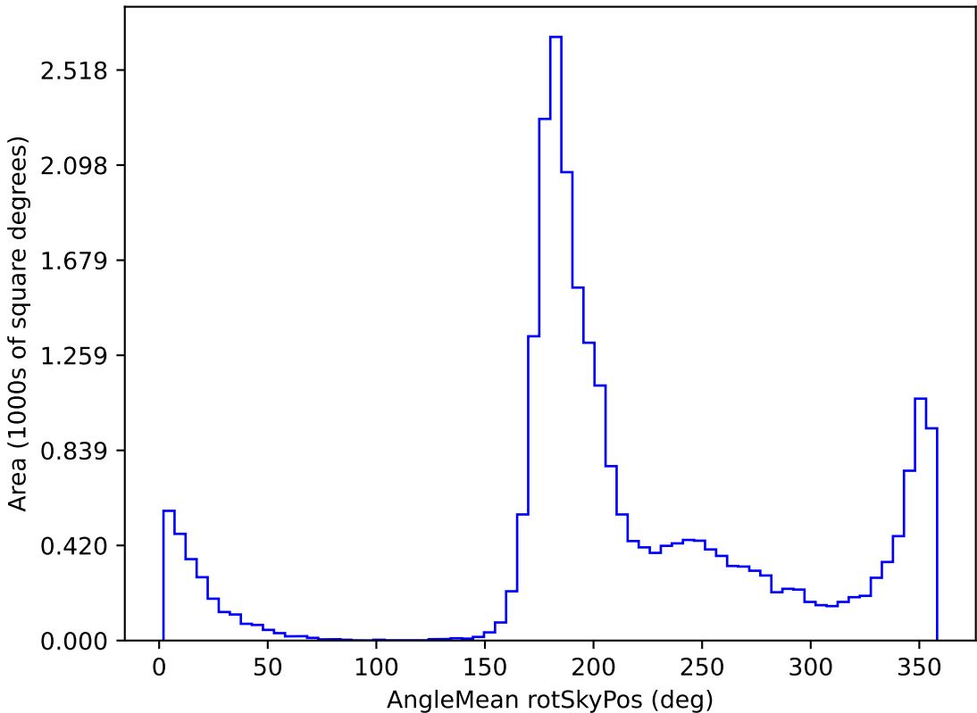
mw_roll_bulge_v3.3_10yrs All sky i band: AngleMean rotSkyPos
