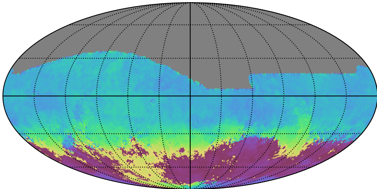
mw_roll_bulge_v3.3_10yrs All sky g band: AngleMean rotSkyPos
