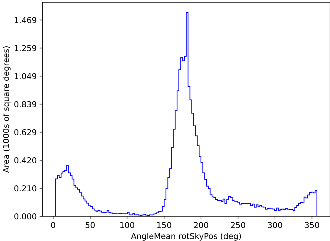
mw_roll_bulge_v3.3_10yrs All sky g band: AngleMean rotSkyPos
