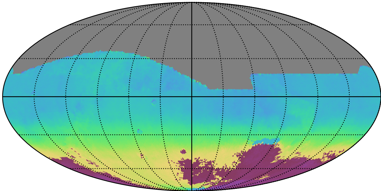
mw_roll_bulge_v3.3_10yrs All sky all bands: AngleMean rotSkyPos
