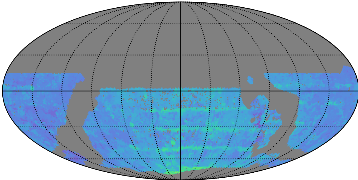
mw_roll_bulge_v3.3_10yrs WFD y band: 80thPercentile Season Length
