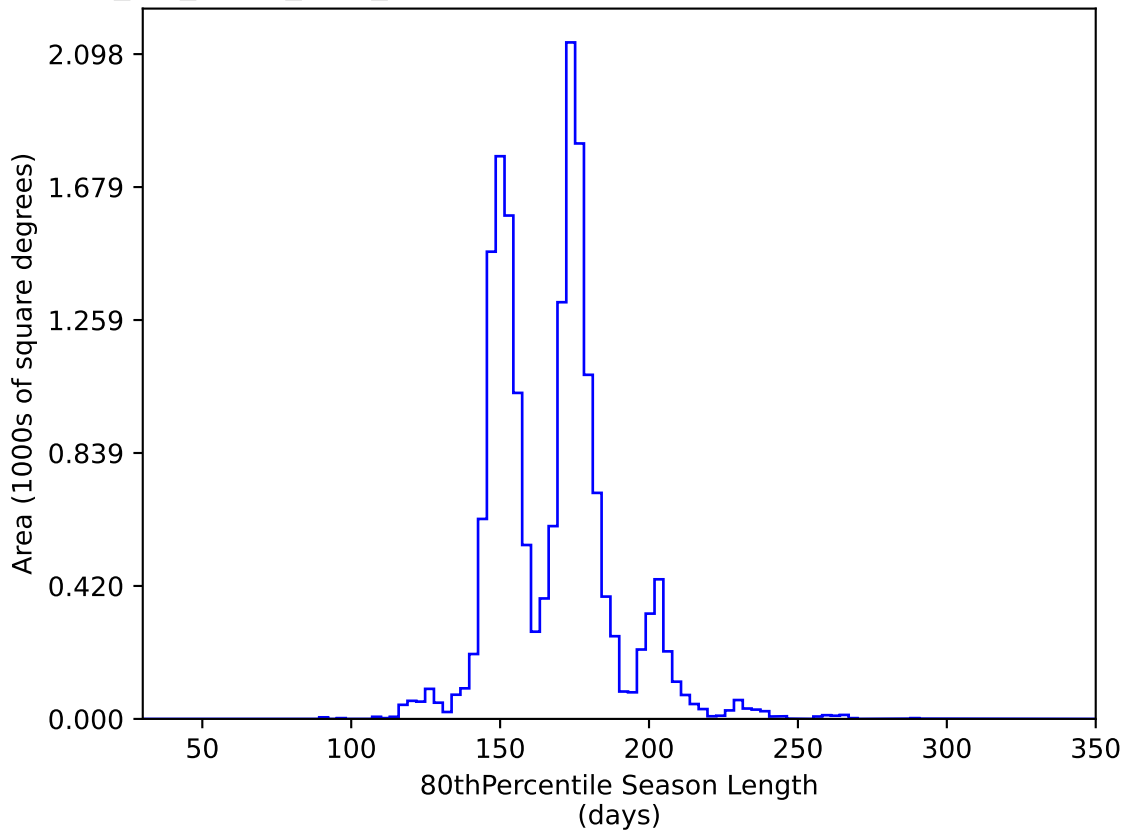
mw_roll_bulge_v3.3_10yrs WFD y band: 80thPercentile Season Length
