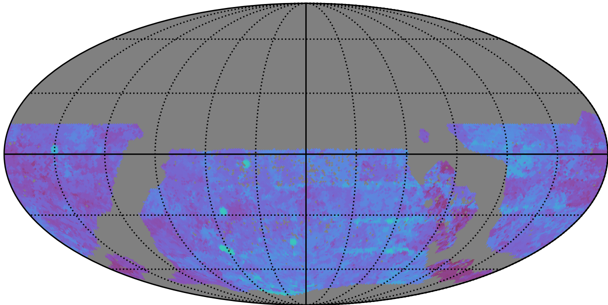
mw_roll_bulge_v3.3_10yrs WFD u band: 80thPercentile Season Length
