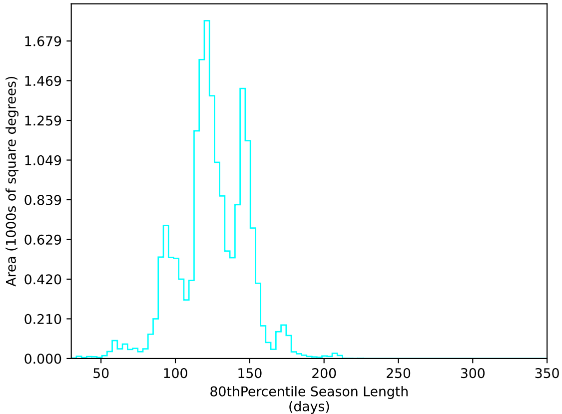
mw_roll_bulge_v3.3_10yrs WFD u band: 80thPercentile Season Length
