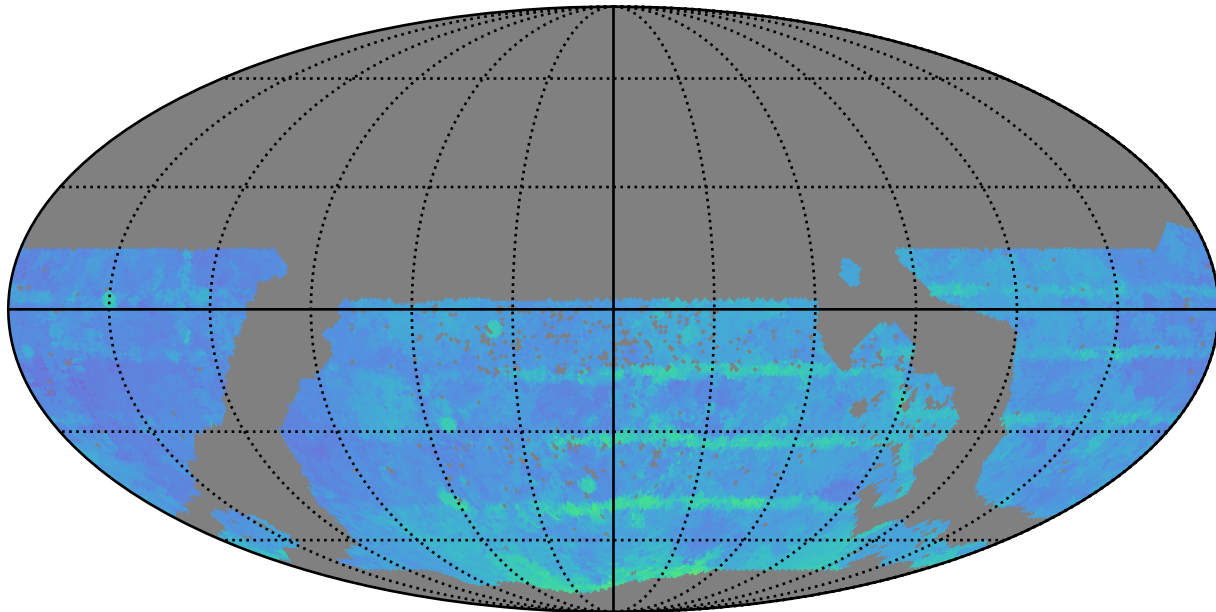
mw_roll_bulge_v3.3_10yrs WFD r band: 80thPercentile Season Length
