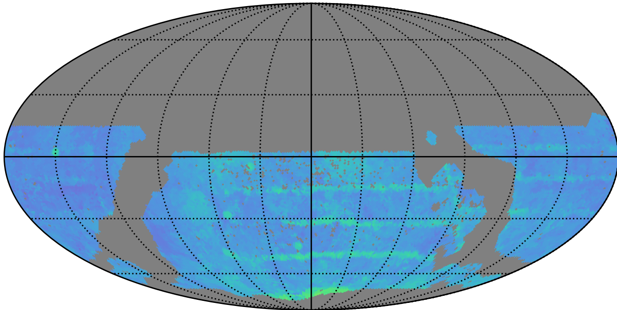
mw_roll_bulge_v3.3_10yrs WFD i band: 80thPercentile Season Length
